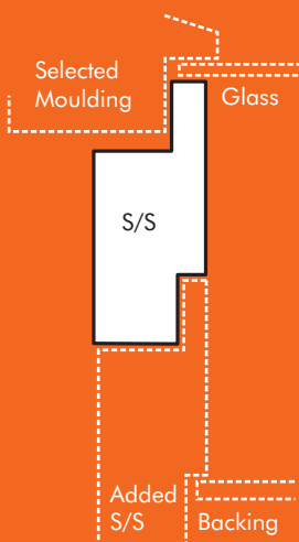
Section view showing use of frame extender for object framing
